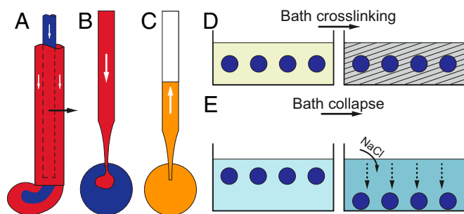
Fig. 3. The generic toolbox of embedded droplet printing allows for complex experimental scheduling to be performed and includes (A) point-of-injection mixing of miscible components via a concentric nozzle, (B) injection of additional fluid after an arbitrary time period after initial printing, and (C) extraction of fluid from incubated droplets. Postprinting, some bath materials may be (D) permanently cross-linked to facilitate handling and characterization, while others may allow for (E) removal of the yield-stress property from the bath material to enable droplet/particle recovery. For the 0.1 wt% Carbopol yield-stress fluid described in this work, the addition of a small amount of NaCl solution triggers a collapse of the microstructure.
